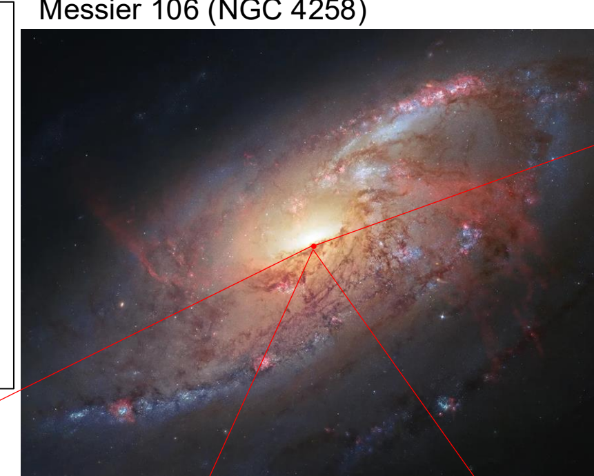
NASA, ESA, the Hubble Heritage Team (STScI/AURA) and R. Gendler (for the Hubble Heritage Team); Acknowledgment: J. Gabor
