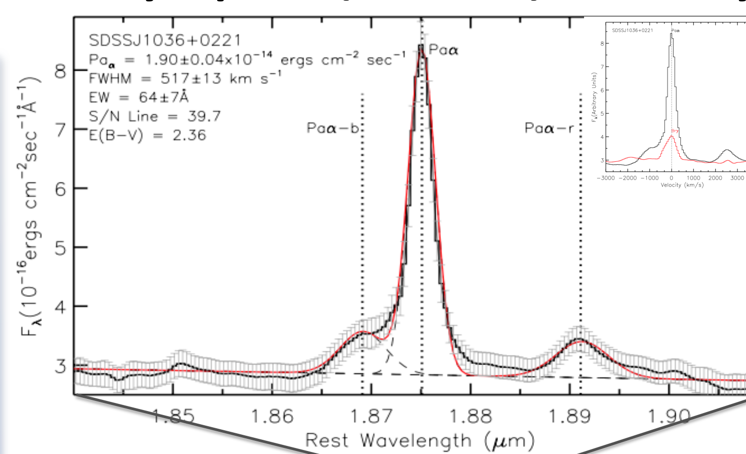
SDSSJ1036+0221: Coalesced object with a rich variety of emission lines. The presence of the [Si X] emission feature is strongly indicative of an AGN. Production of this line requires a spectral energy distribution that can only be provided by accretion onto a SMBH. Its H_2 /Bry line flux ratio is consistent with an AGN nature. The 10 pixel extraction corresponds to 2.5 kpc at the redshift of the target.
