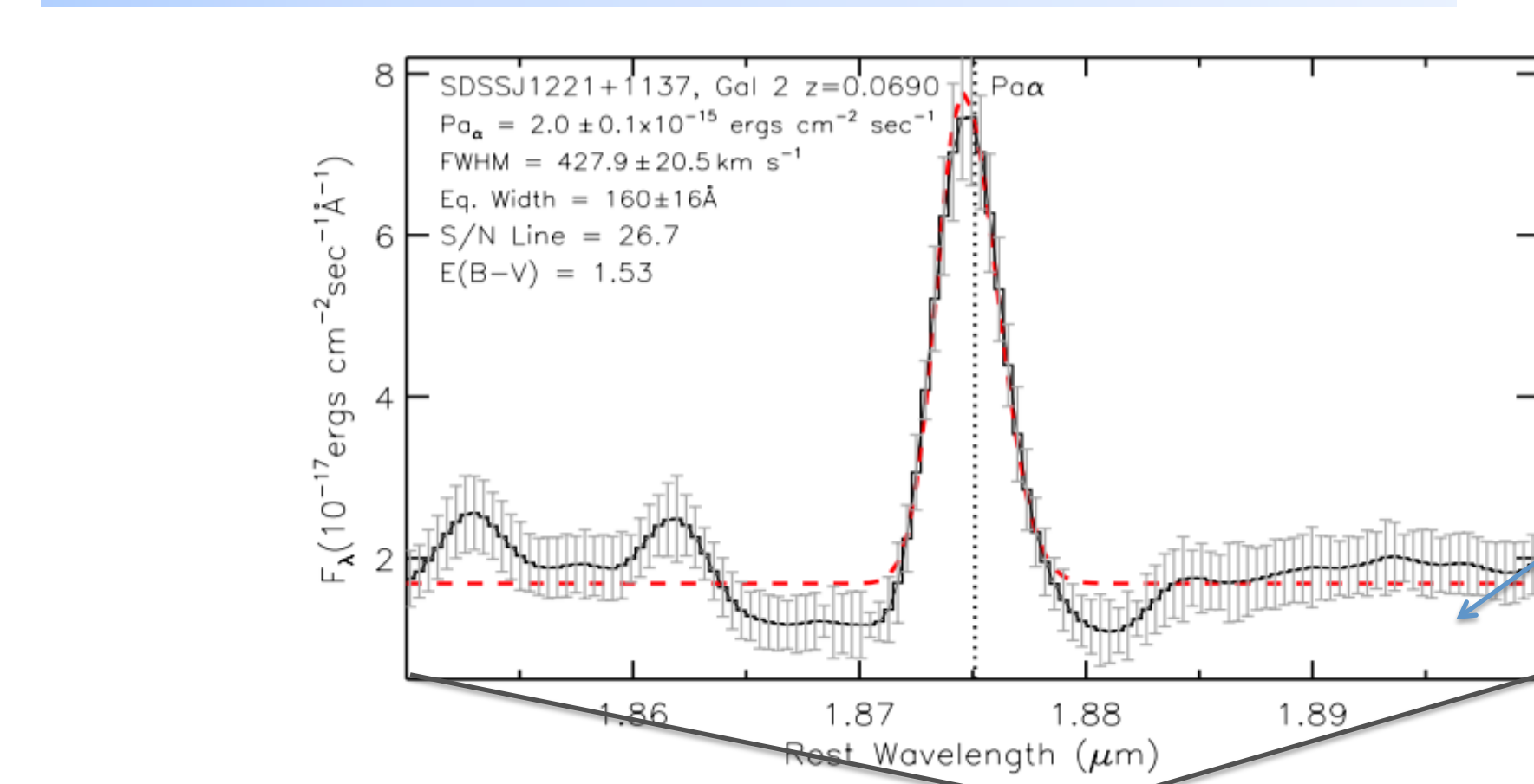
SDSSJ1221+1137: Galaxy 2 is classified as an AGN using the near-IR line-ratio diagnostic diagram. [Si VI] emission is also present in galaxy 2, which lends credibility to an AGN being the dominant excitation mechanism. Both galaxies use a 4 pixel extraction, which corresponds to 1.3 kpc at the target's redshift.
