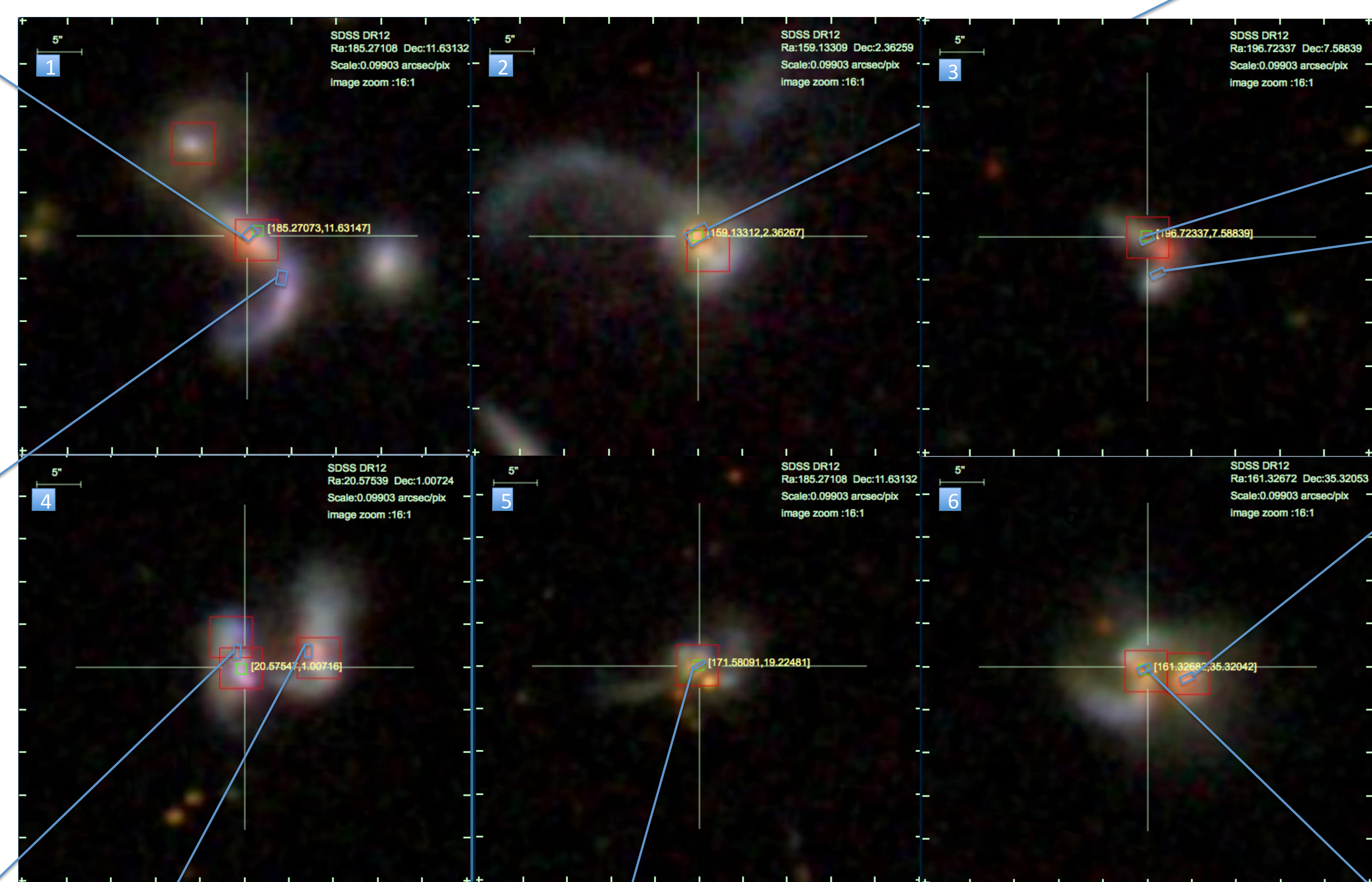
SDSSJ1221+1137: Galaxy 2 is classified as an AGN using the near-IR line-ratio diagnostic diagram. [Si VI] emission is also present in galaxy 2, which lends credibility to an AGN being the dominant excitation mechanism. Both galaxies use a 4 pixel extraction, which corresponds to 1.3 kpc at the target's redshift.
